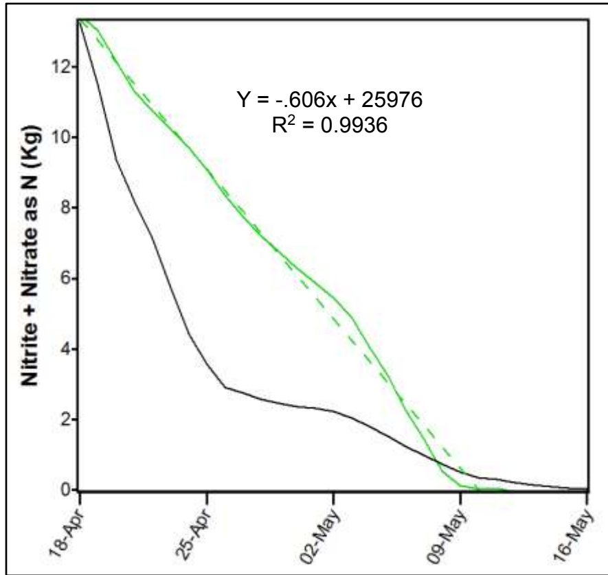
Figure 5.5. Daily NO 3 - -N load detected by sensor (green) plotted against an estimated denitrification first order decay (black).
